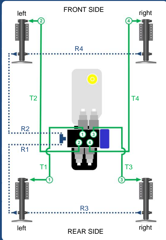
Situation 1 : 8 hoses
