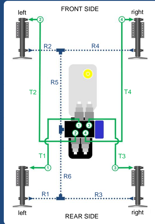
Situation 2 : 10 hoses
